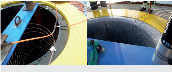
Grouting of joint between steel structure and concrete transition piece (TP) - Offshore at Nissum Bredning
